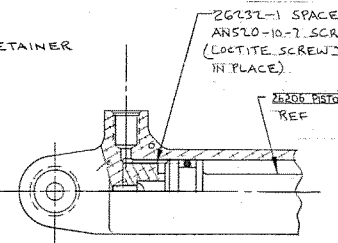
ⓐ DETAIL A APPLIES -5 ASSY ONLY
